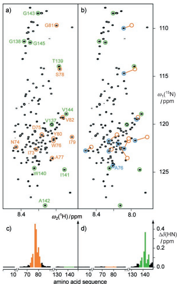
Figure 1. NMR spectroscopy data showing the impact of single amino acid replacements in the hydrophobic clusters identified in OmpX unfolded in 8 M urea solution. a), b) 2D [ ^{15}\text{N} , ^1\text{H} ]-HSQC NMR spectra of wild-type OmpX and OmpX[W76A], respectively; orange and green circles mark the positions of the backbone ^{15}\text{N} - ^1\text{H} resonances of the hydrophobic clusters I (residues 73–82 in the 148-residue polypeptide) and II (residues 137–145), respectively, in the wild-type protein. In (b), additional blue circles mark the resonances of residues 73–82 in OmpX[W76A], and corresponding orange and blue circles are connected by orange lines. c) The chemical shift differences \Delta\delta(^{15}\text{N}, ^1\text{H}) between corresponding amide groups in OmpX[W76A] and OmpX are plotted versus the amino acid sequence, where the data for the clusters I and II are colored orange and green, respectively. No data is presented for residues 11 to 63 and 91 to 129, which show no chemical shift changes. d) Same as (c) for OmpX[W140A].
